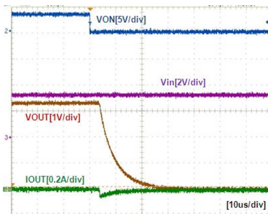
Figure 21. Turn-Off Response ( V_{IN}=3.3\text{ V} , C_{IN}=1\text{ }\mu\text{F} , C_{OUT}=0.1\text{ }\mu\text{F} , R_L=500\text{ }\Omega , FPF1204 / 45)
