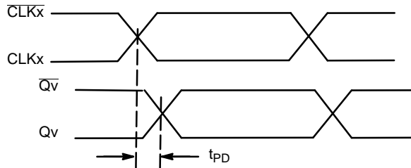
Figure 12. Propagation Delay
