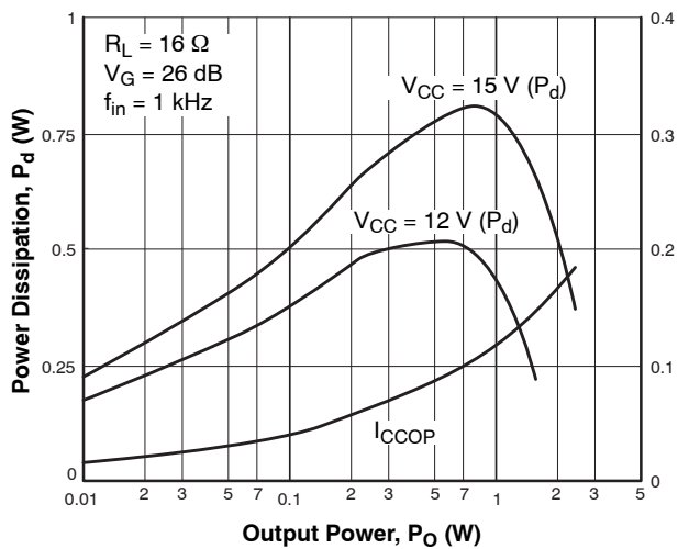
Figure 26. P_d - P_O
