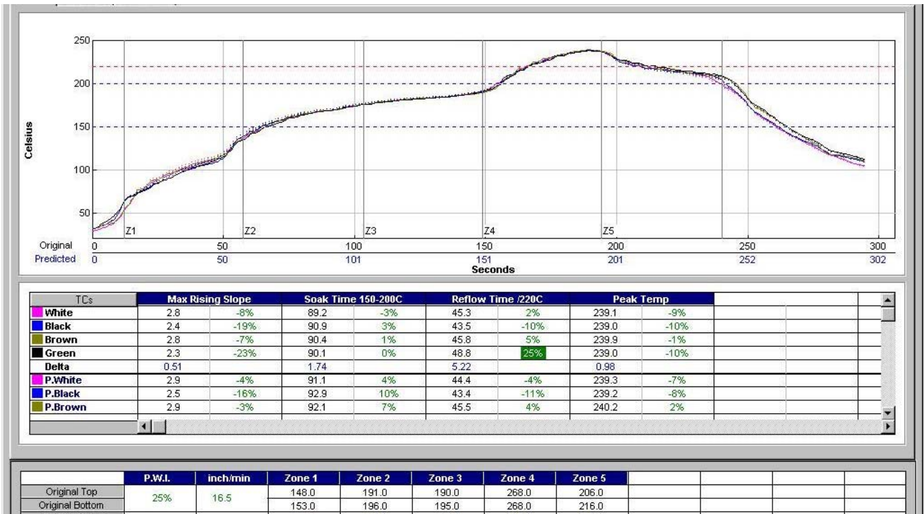
Figure 5. Reflow Profile used for Building Demonstration Boards
