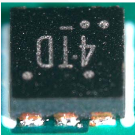
Figure 1. Exposed Copper on Package Edge, Solder Wetting after Reflow, from Singulation Process
