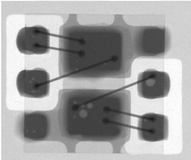
Figure 3. X-Ray Image Showing Voiding Caused by Normal Process Variation during Reflow
