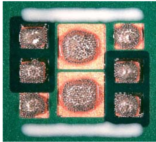
Figure 2. Printed Solder Paste, Recommended Print
