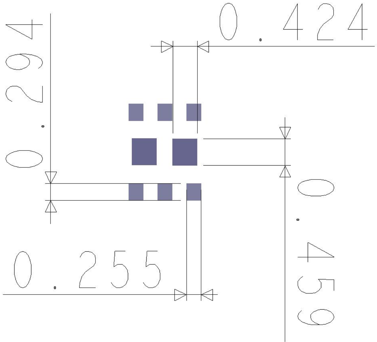
Figure 4. Solder Stencil Opening Recommendations (mm)
