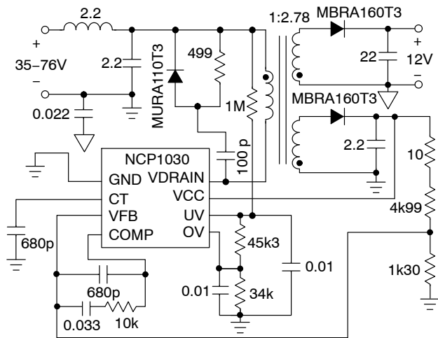
Figure 12. Complete Circuit Schematic
