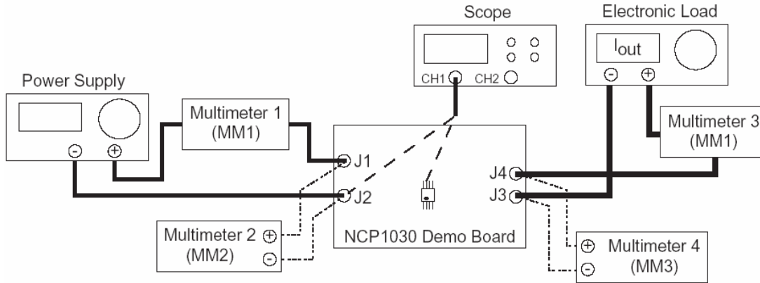
Figure 22. Test Setup
