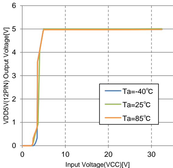
Fig7. [VDD] Vo vs. Input Voltage
