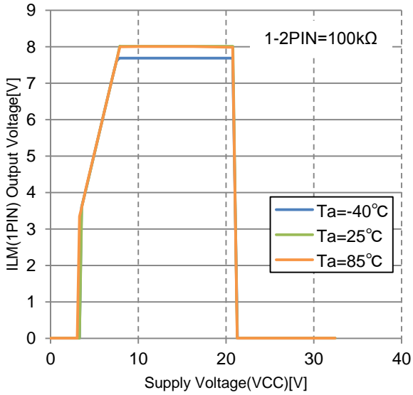
Fig24. [ILM(8V)] Vo vs. Input Voltage
