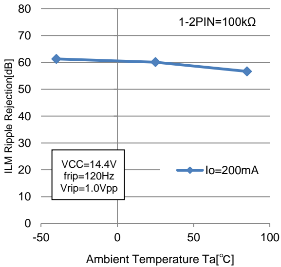
Fig28. [ILM(8V)] Ripple Rejection vs. Ta
