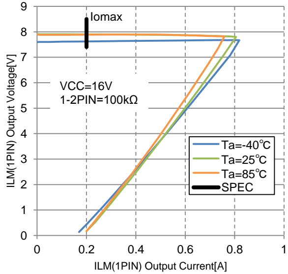
Fig27. [ILM(8V)] Vo vs. Io@VCC=16V
