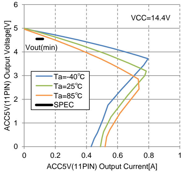
Fig48. [ACC5V] Vo vs. Io@VCC=14.4V
