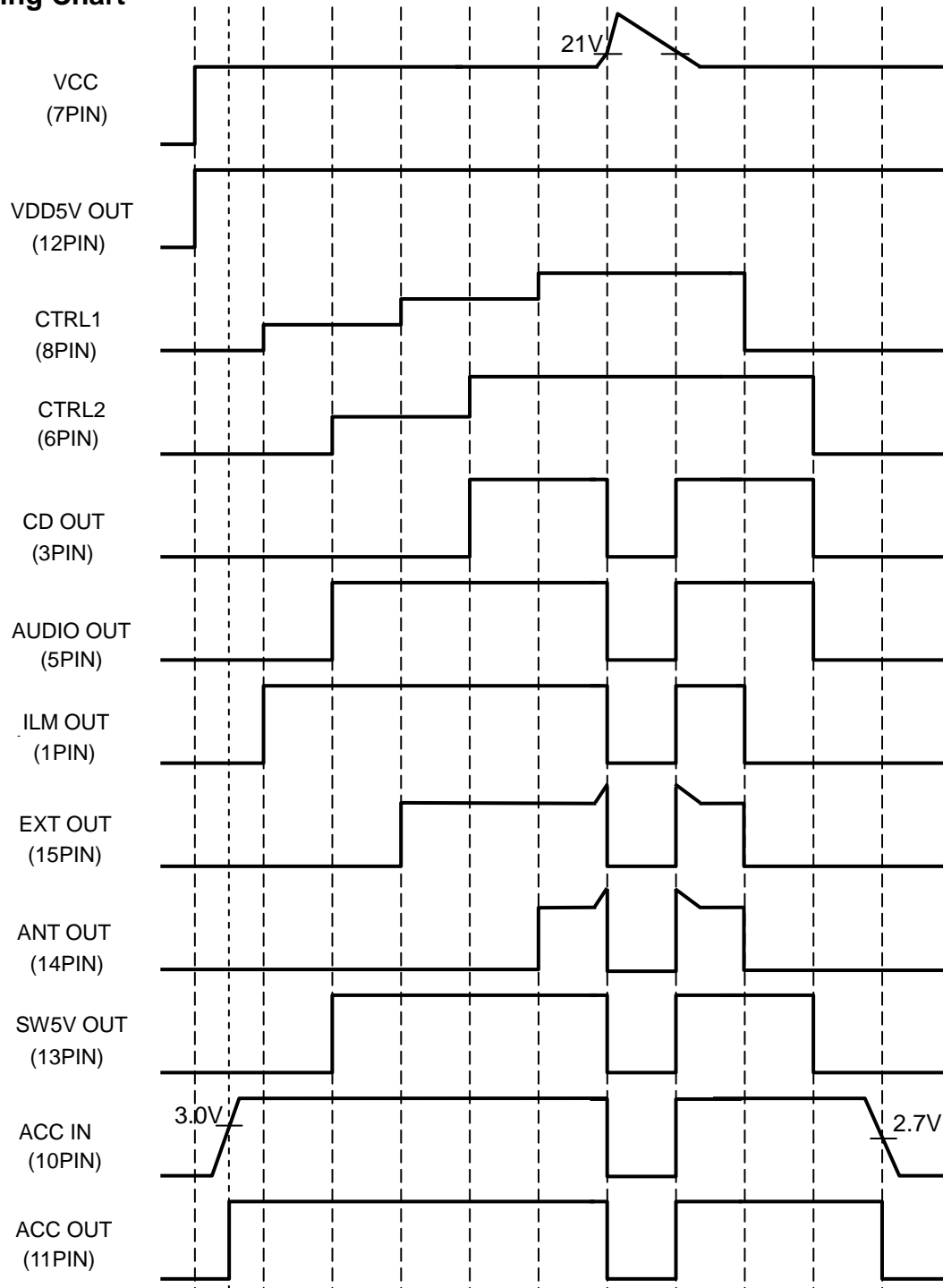
Fig6. Timing Chart
