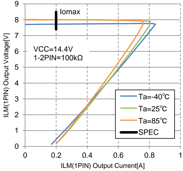
Fig25. [ILM(8V)] Vo vs. Io@VCC=14.4V
