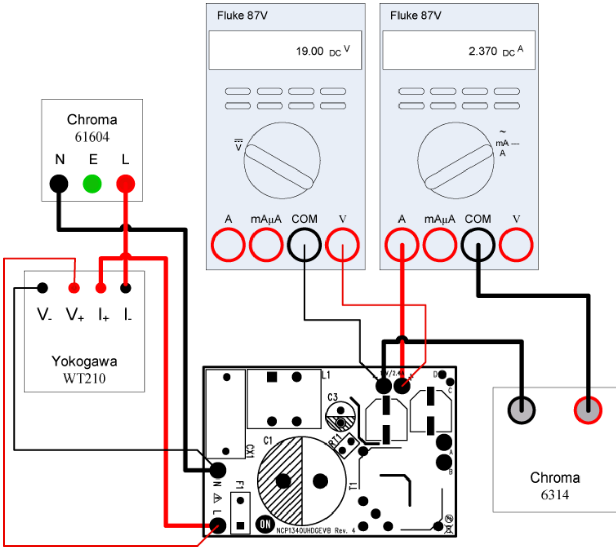
Figure 1: Test Setup
