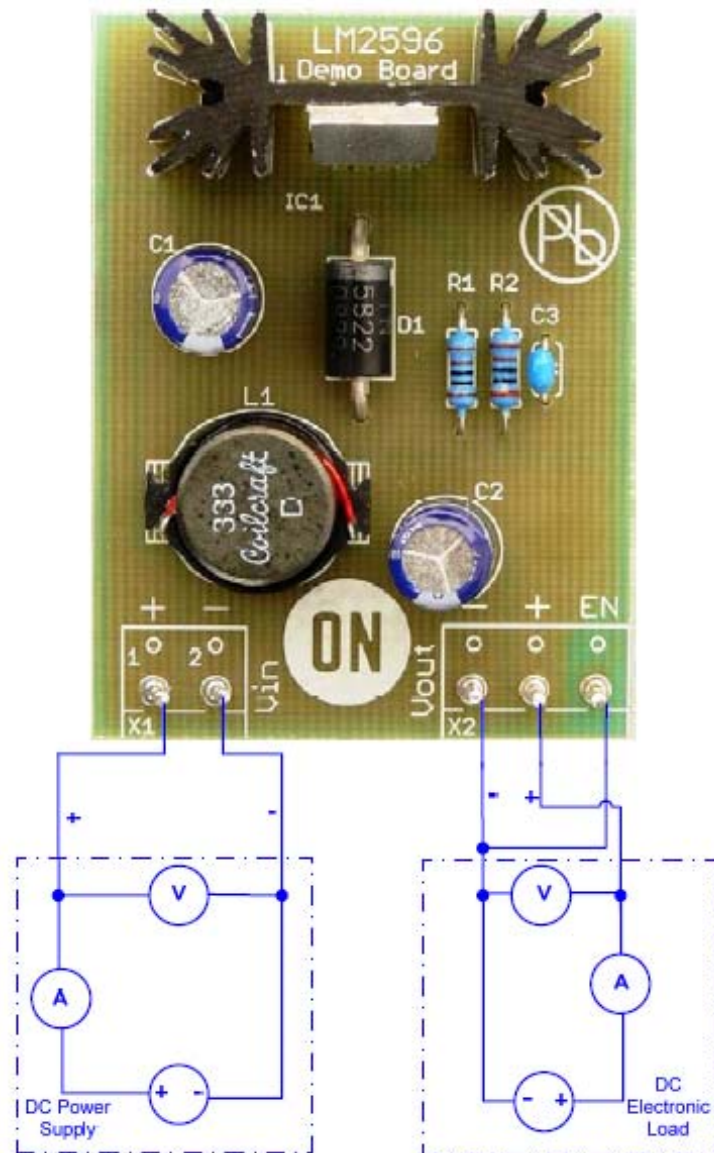
Figure 1: Test Setup
