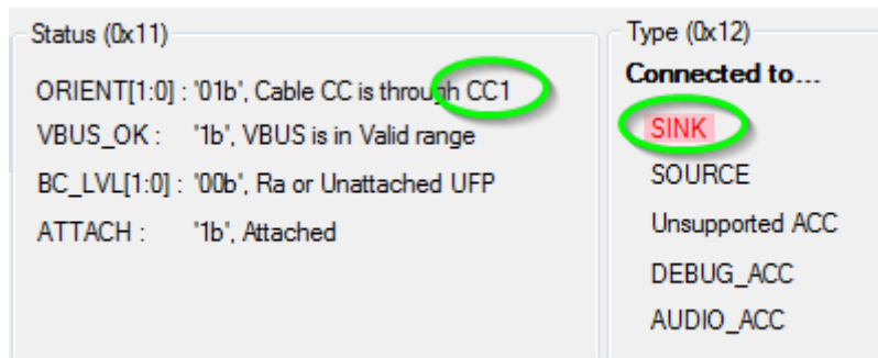
Figure 6 – CC termination after initial attach
