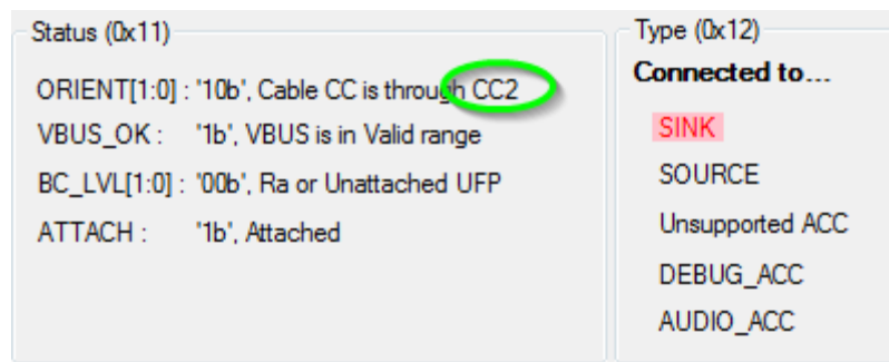
Figure 7 - CC termination after flip
