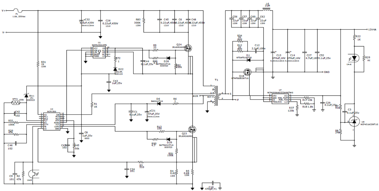
Figure 2. Circuit Schematic
