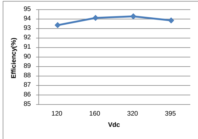
Figure 6. Efficiency
