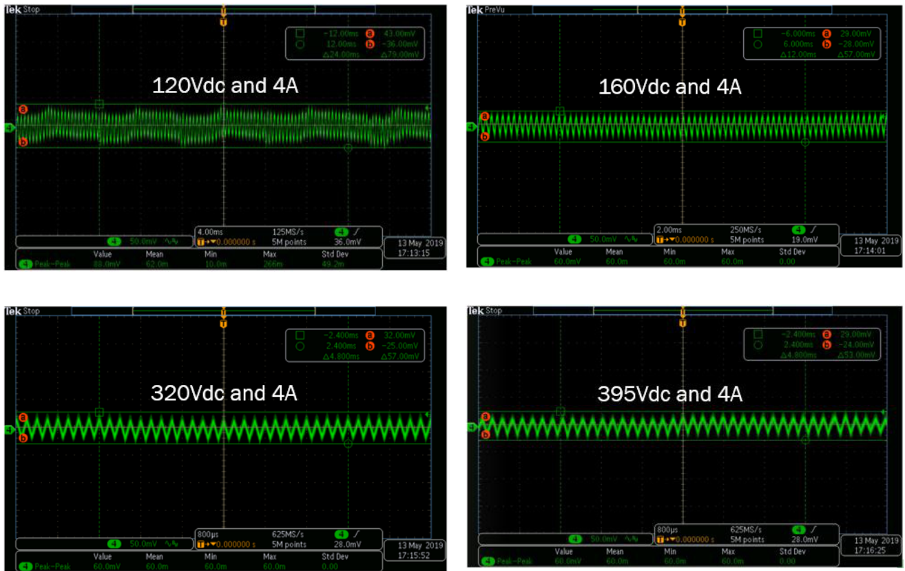
Figure 9. Output Ripple at Full Load
