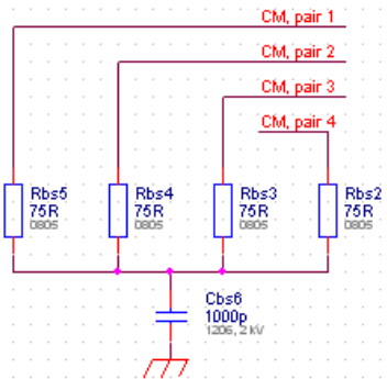
Figure 6. Bob-Smith Termination
