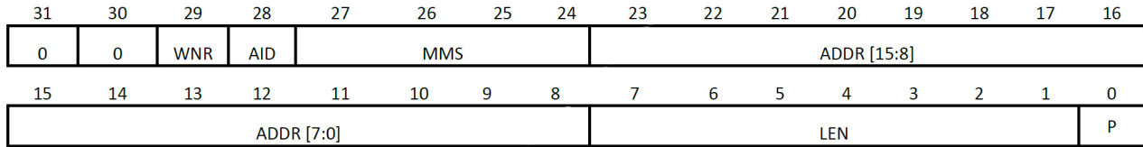
Figure 2. Control Command Format
