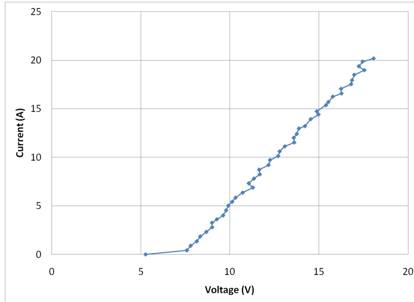
Figure 4. Sample TLP Curve of a TVS Diode
