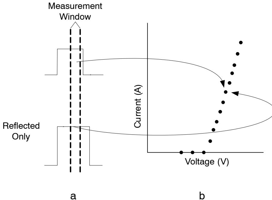
Figure 3. Explanation of How I-V Points are Determined from the TLP Pulses
