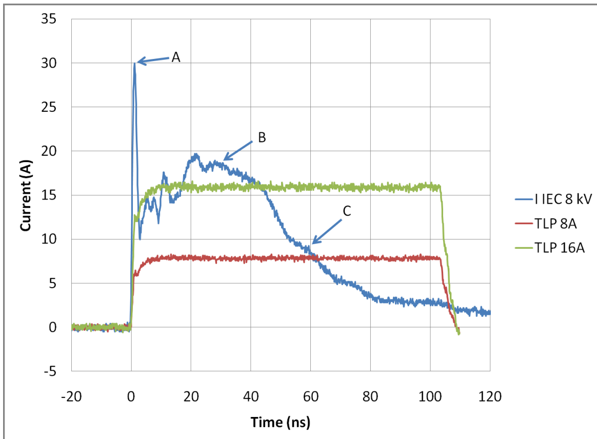
Figure 1. Comparison of a Current Waveform of IEC 61000-4-2 with TLP Pulses at 8 and 16 A
