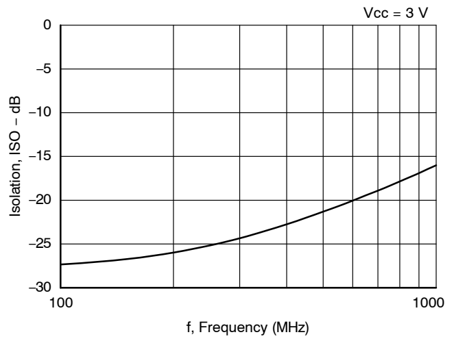
Figure 4. Isolation
