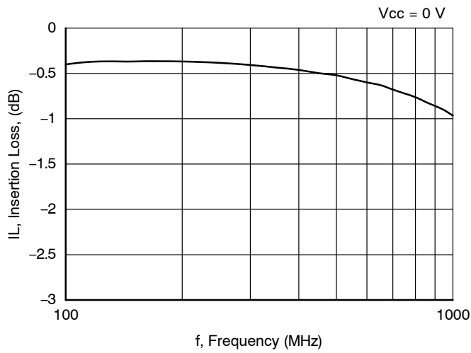
Figure 3. Insertion Loss
