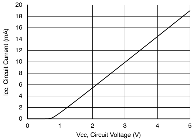
Figure 5. Icc - Vcc
