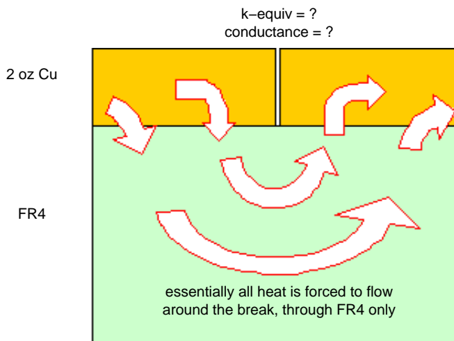
Figure 13. A Discontinuous Spreader Plane
