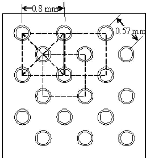
Figure 7. Possible 18-via Pattern for NCS5651
