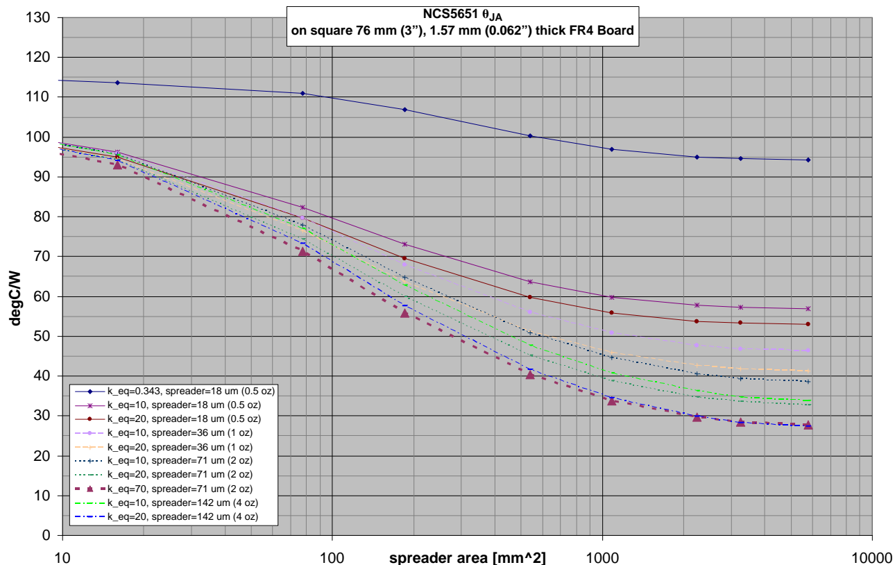
Figure 5. \theta_{JA} of NCS5651 on Square 76 mm (3"), 1.57 mm (0.062") Thick FR4 board
