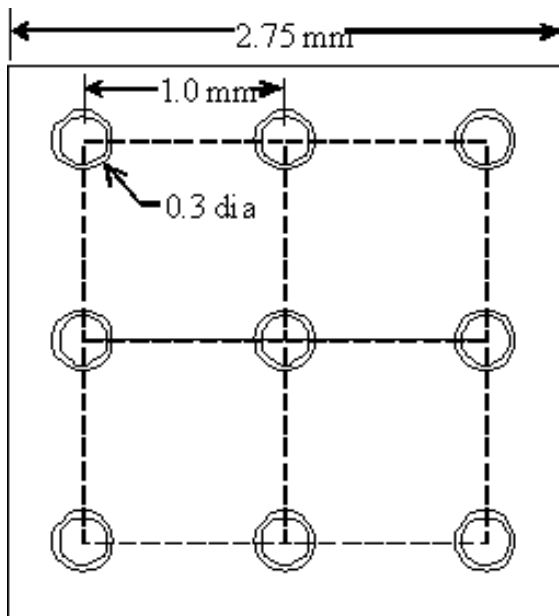
Figure 6. Possible 9-via Pattern for NCS5651
