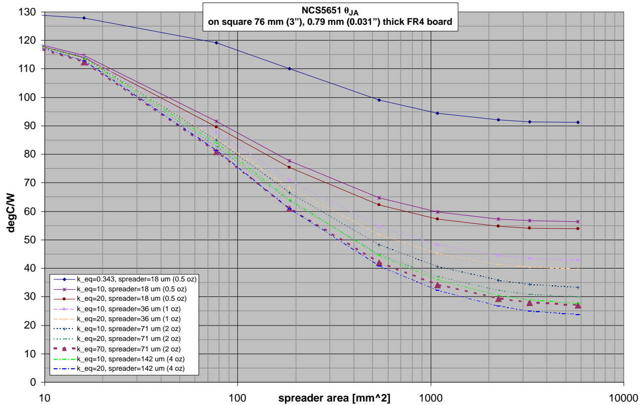
Figure 4. \theta_{JA} of NCS5651 on Square 76 mm (3"), 0.79 mm (0.031") Thick FR4 board
