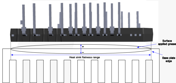
Figure 3. Measurement Point of Heat Sink Flatness
