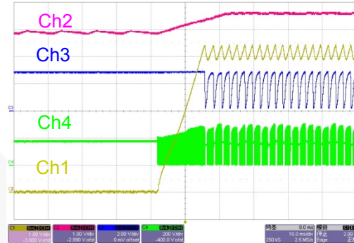
Figure 39. 120 V AC / 60 Hz at Max. Load, Disable (Ch 1: V O , Ch 2: V CC , Ch 3: V FB , Ch 4: V DS )
