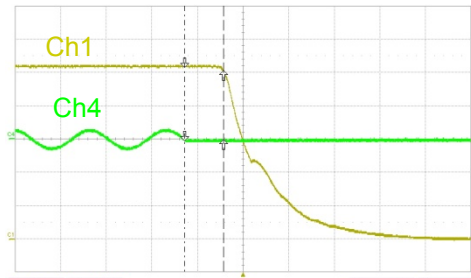
Figure 29. 85 V AC / 60 Hz at Max. Load (Ch 1: V O , Ch 4: V AC )
