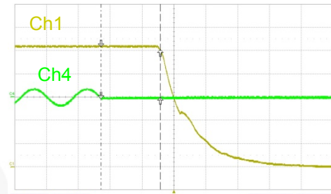
Figure 30. 115 V AC / 60 Hz at Max. Load (Ch 1: V O , Ch 4: V AC )
