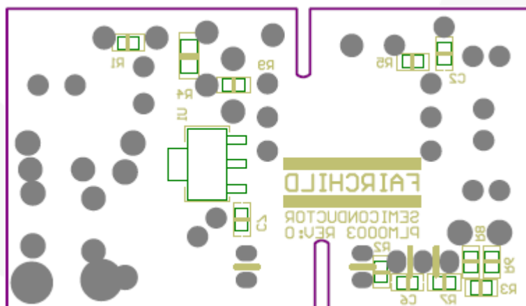
Figure 4. Bottom Overlay Silk Screen
