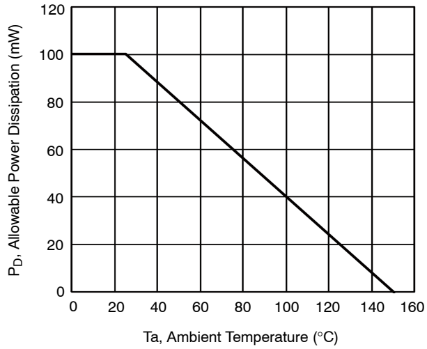
Figure 9. P_D - T_a
