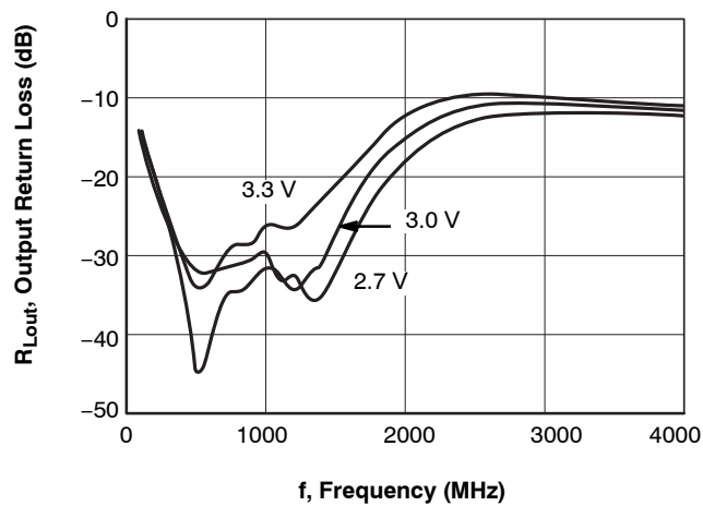
Figure 7. R_{Lout} - f
