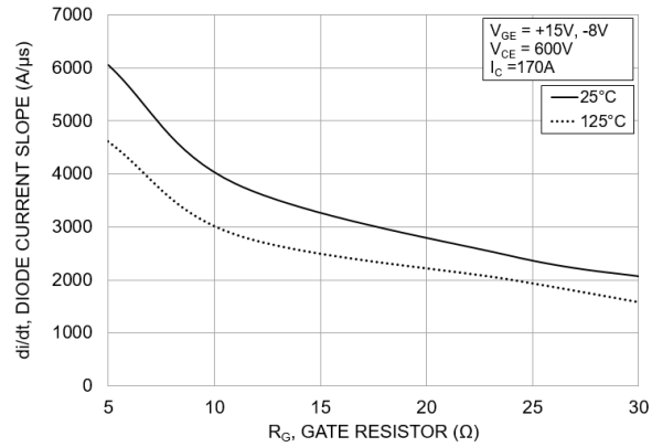
Figure 40. Typical di/dt vs. R_G
