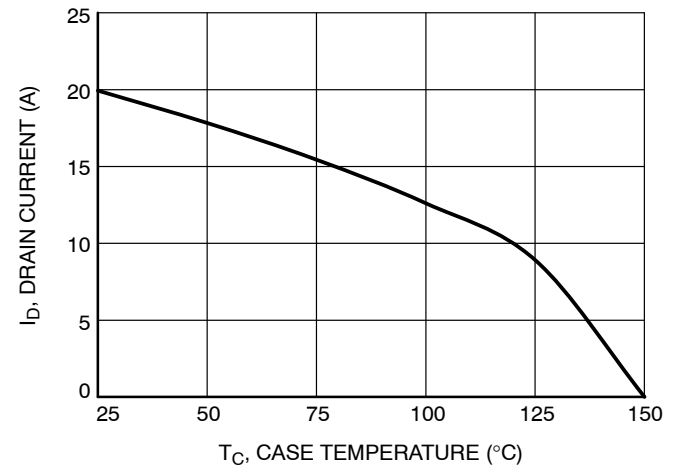
Figure 10. Maximum Drain Current vs. Case Temperature
