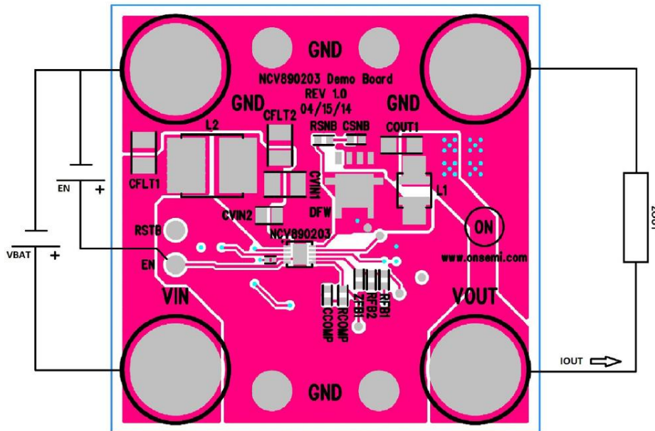
Figure 5. NCV890203 Board Connections
