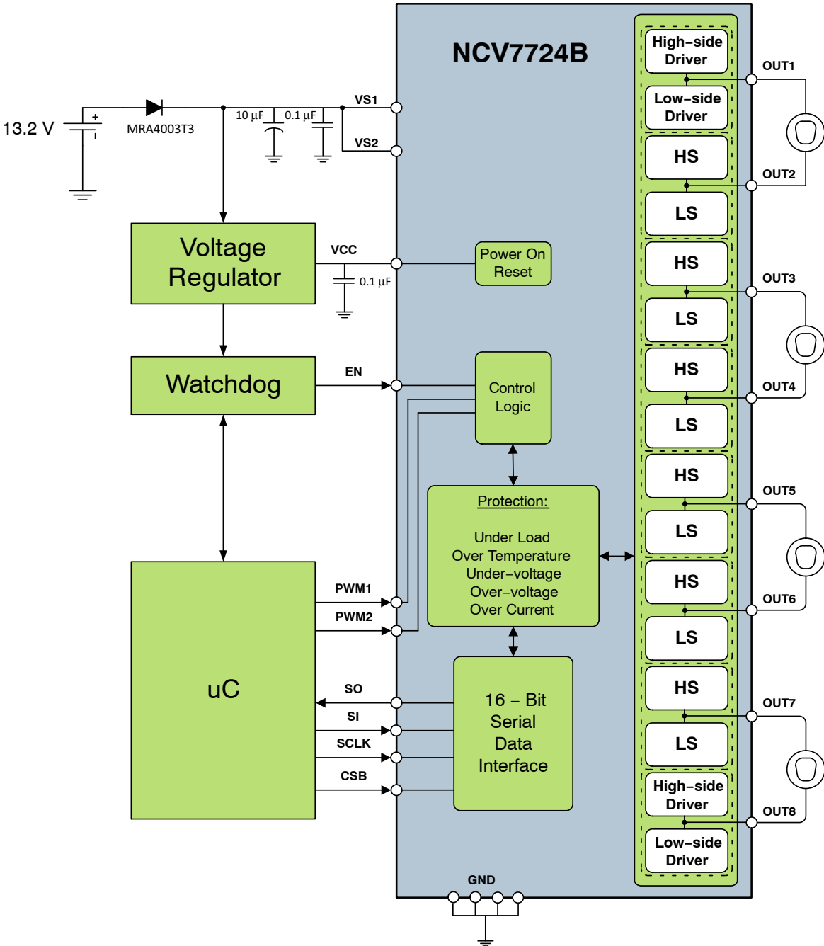
Figure 1. Typical Application
