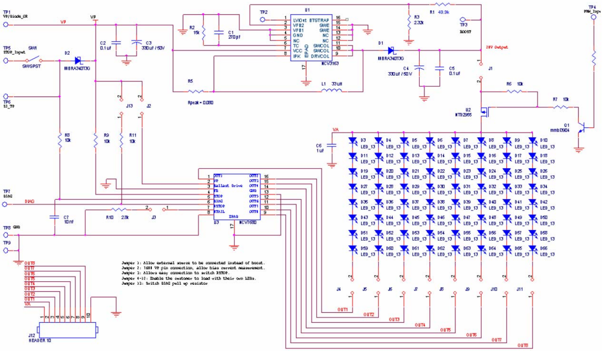
NCV7680_NCv3163_EVB Schematic REV 1
