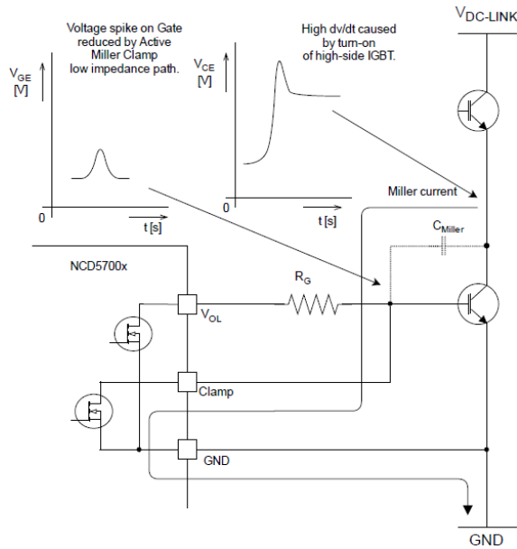
Figure 7. Current Path without Miler Clamp Protection
