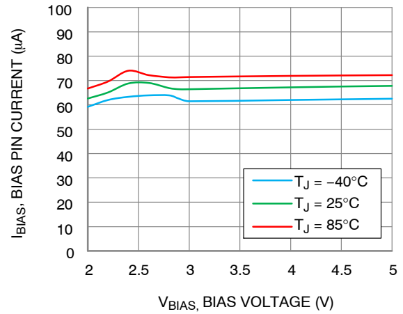
Figure 4. BIAS Pin Current vs. V_{BIAS} and T_J
