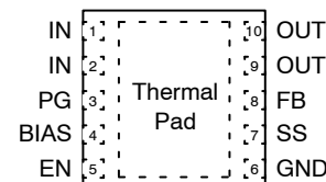
DFN10-3x3-0.5P
