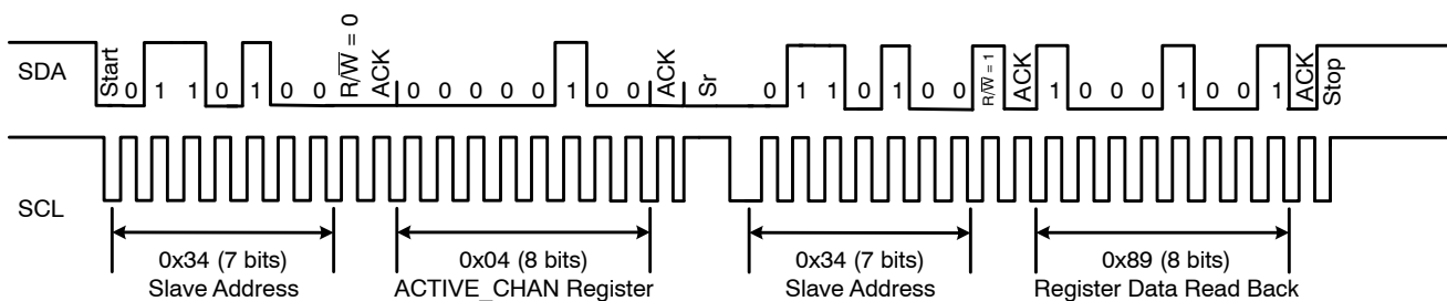
Figure 4. I 2 C Register Read with Repeated Start Example
