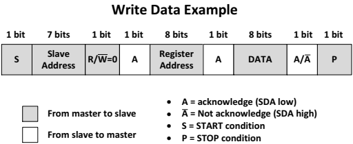
Figure 6. I 2 C Write Protocol Format
