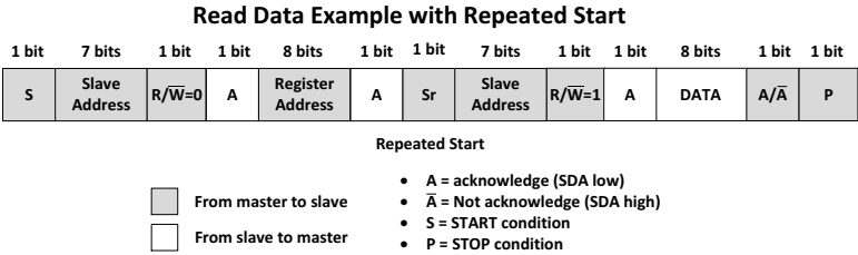
Figure 7. I 2 C Read with Repeated Start Format
