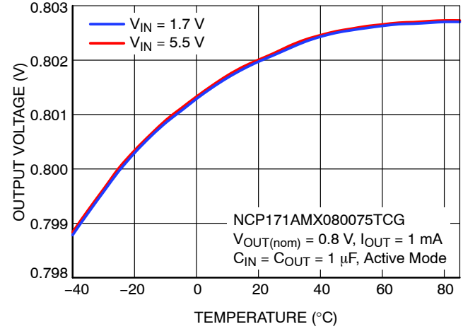
Figure 23. Output Voltage vs. Temperature in Active Mode
