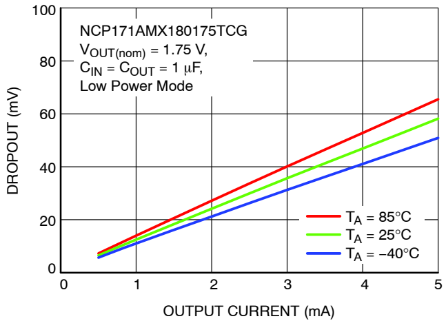
Figure 44. Dropout vs. Output Current in Low Power Mode
