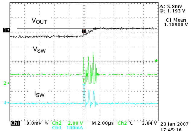
Figure 27. PFM Switching Waveforms (V_{IN} = 3.6 \text{ V}, V_{OUT} = 1.2 \text{ V}, I_{OUT} = 0 \text{ mA}, \text{Temperature} = 25^\circ\text{C})
