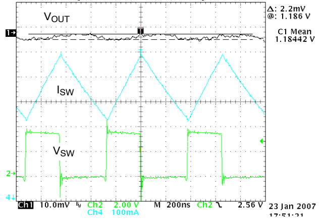
Figure 26. PWM Switching Waveforms (V_{IN} = 3.6 \text{ V}, V_{OUT} = 1.2 \text{ V}, I_{OUT} = 600 \text{ mA}, \text{Temperature} = 25^\circ\text{C})
