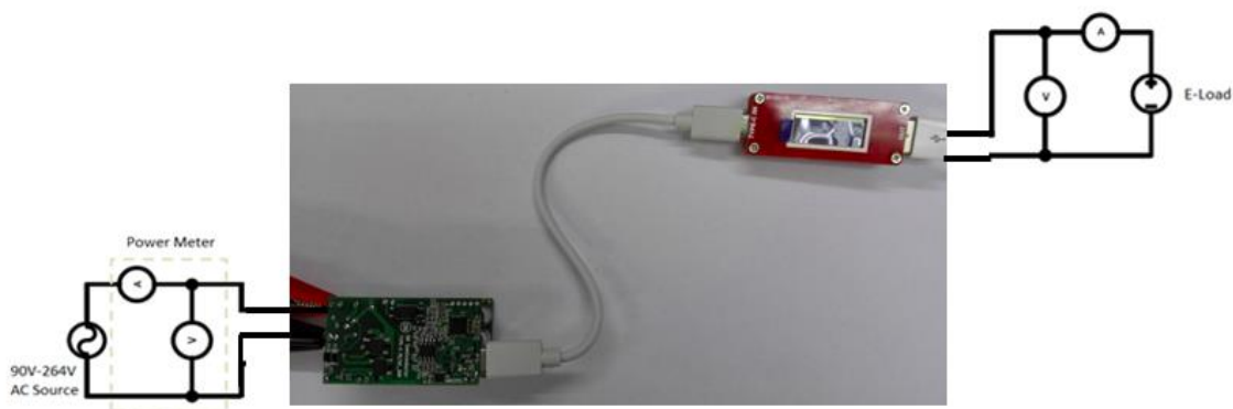
Figure 1: PD Test Setup for 45W PD/QC Demoboard
