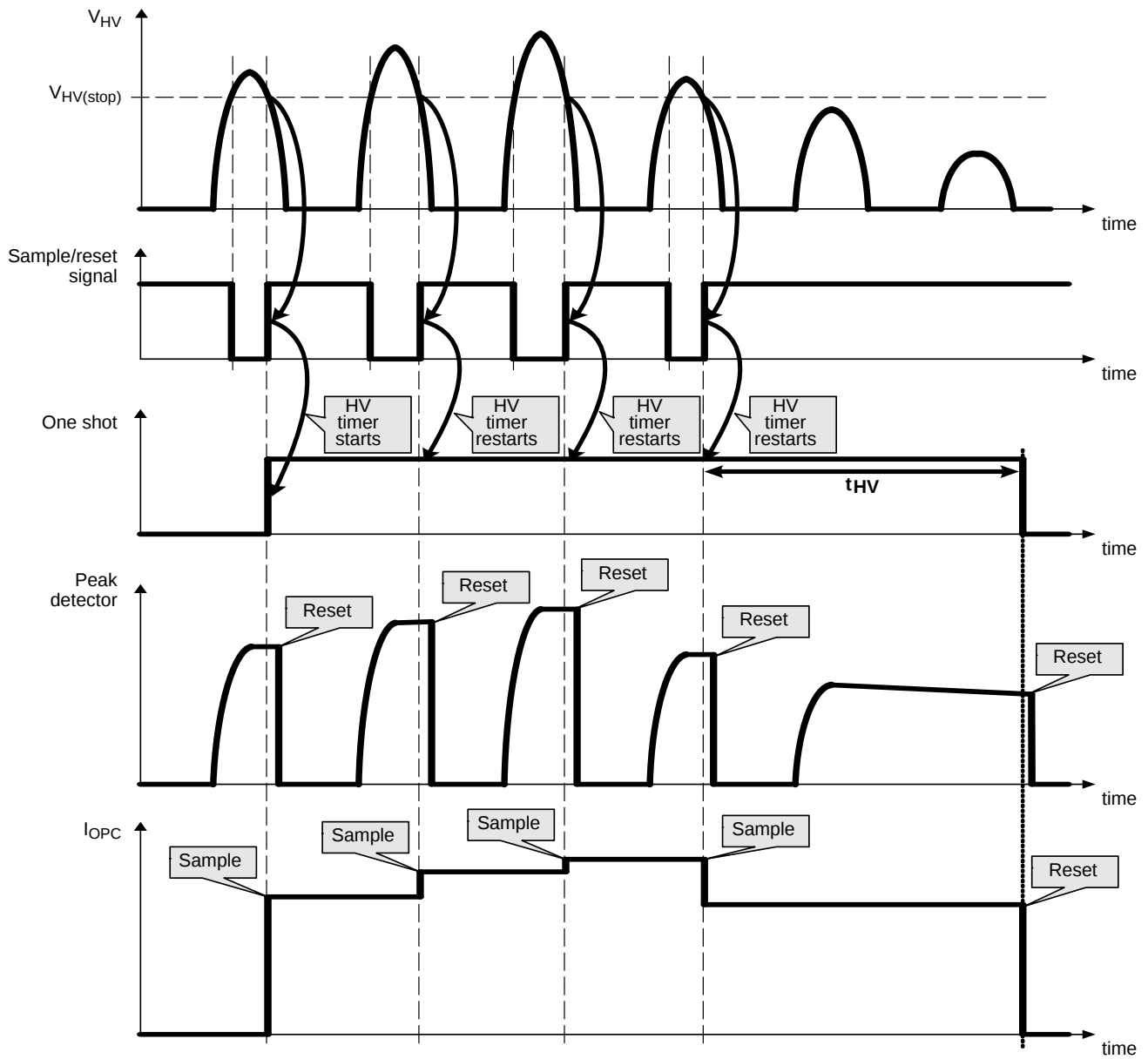
Figure 40. Overpower Compensation
