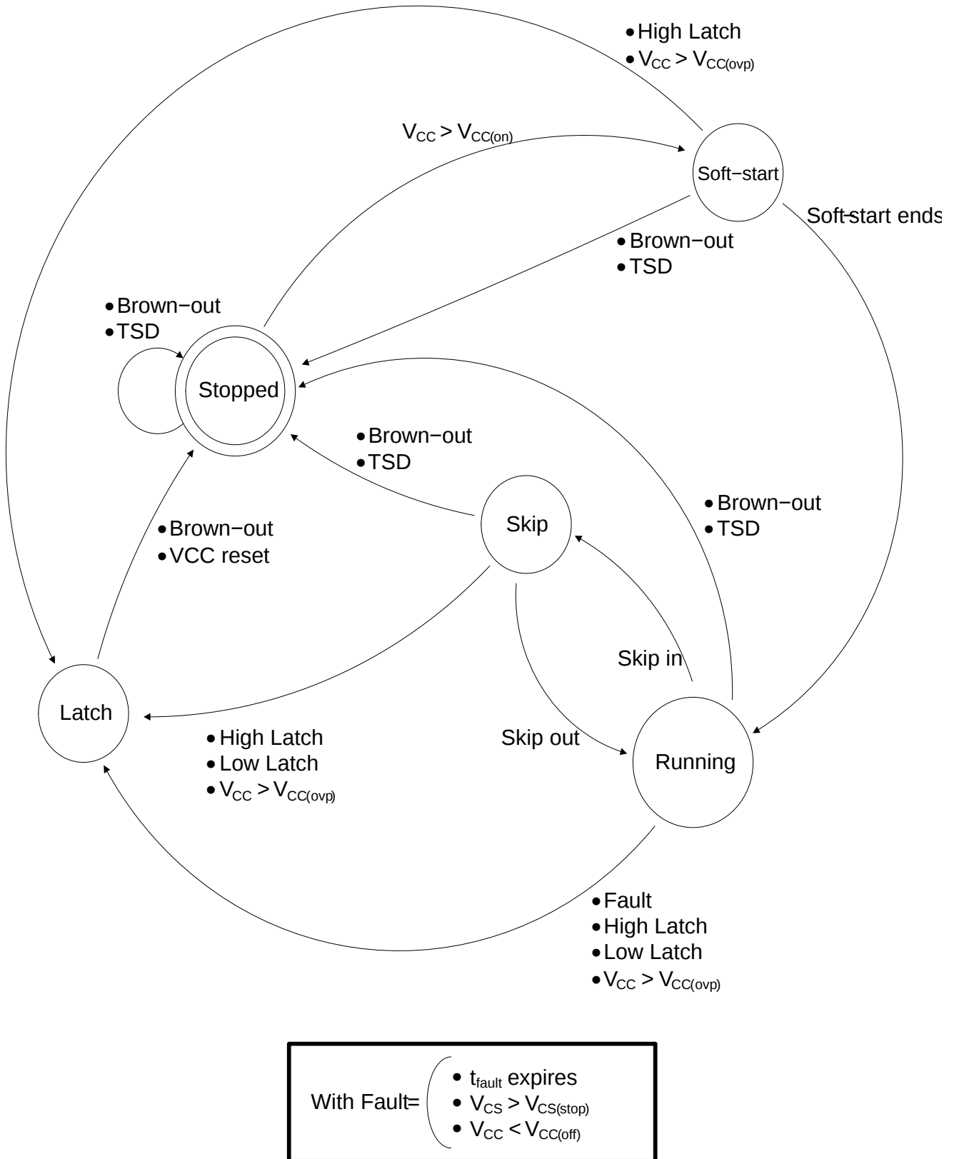
Figure 52. Controller Operation State Diagram (Latched Protection)
