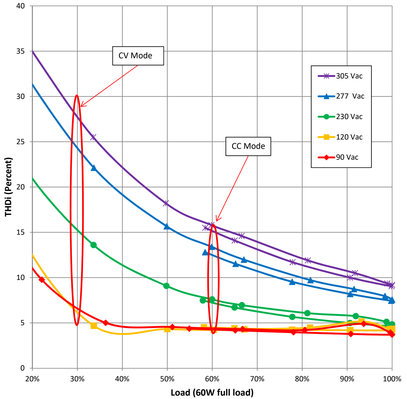
Figure 8. THDi Performance
