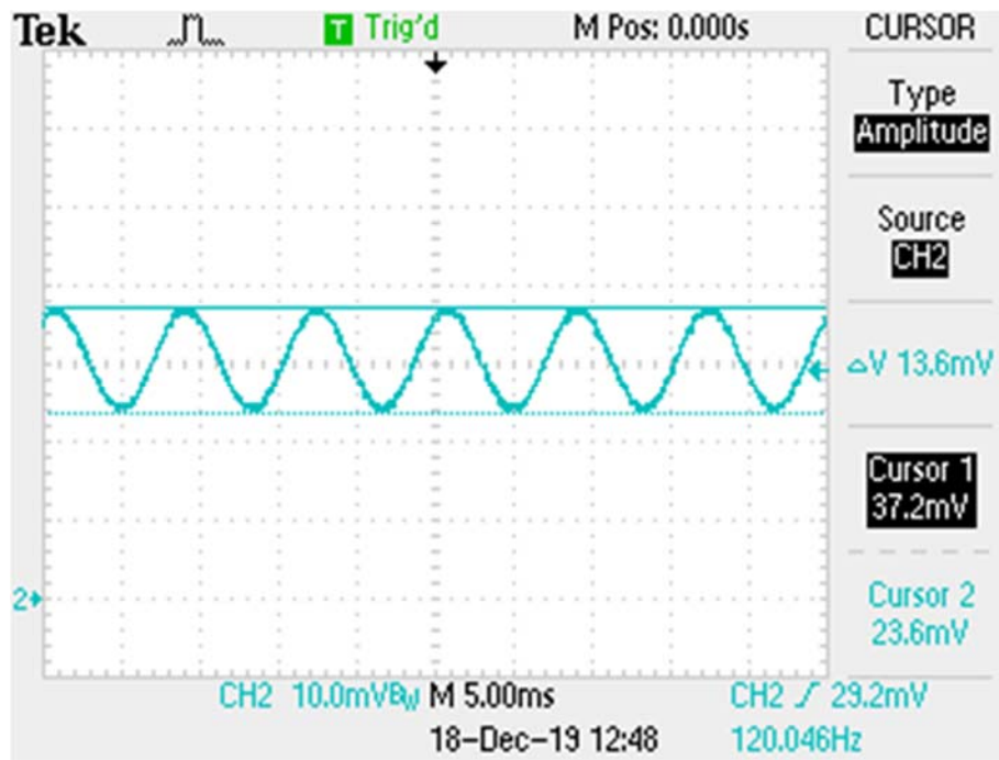
Figure 13. Output Ripple Current with 230 V ac Input
