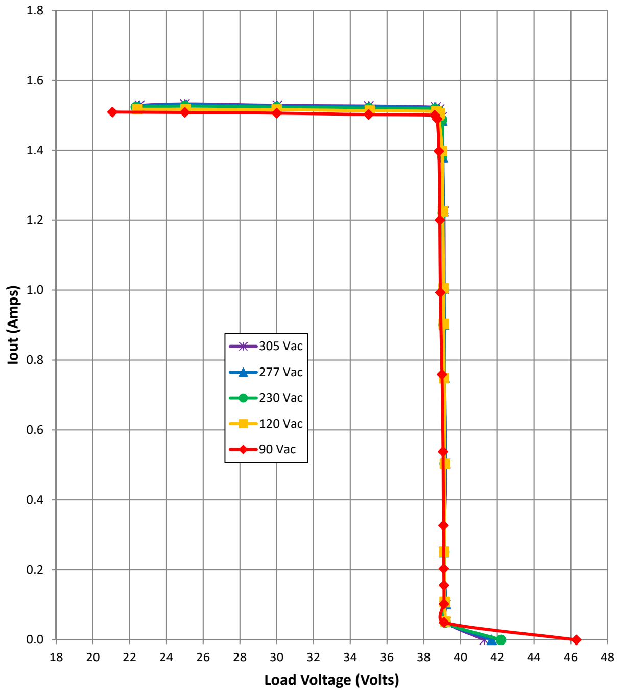
Figure 6. Line and Load Regulation Performance
