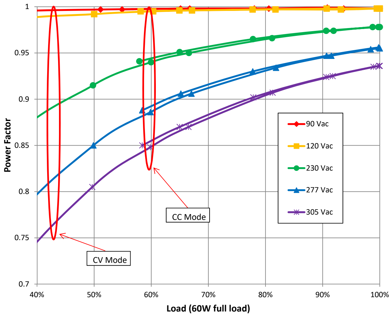
Figure 5. Power Factor Performance
