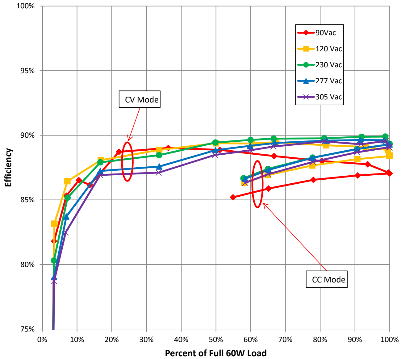
Figure 9. Efficiency
