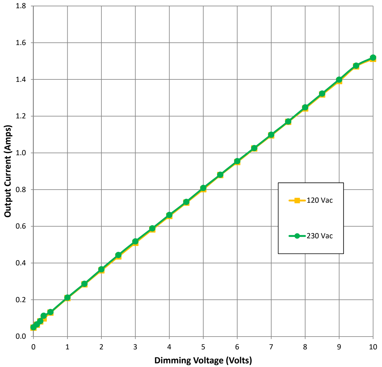
Figure 7. Dimming Performance
