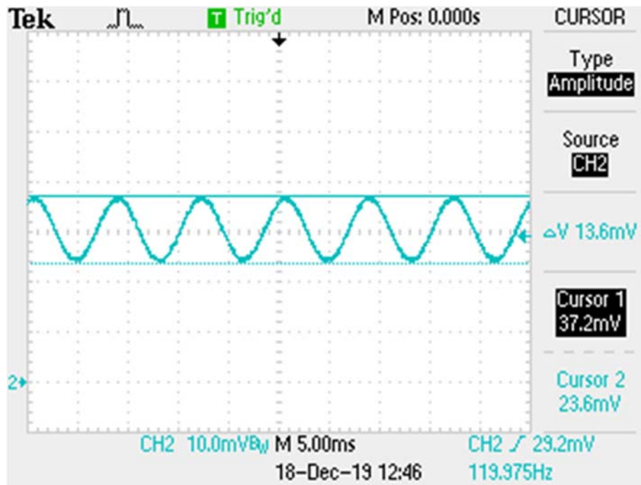
Figure 12. Output Ripple Current with 120 V ac Input
