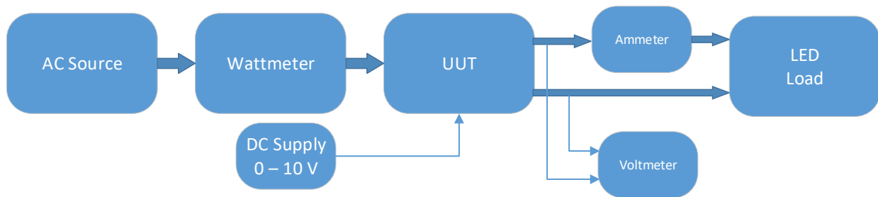
Figure 4. Test Setup
