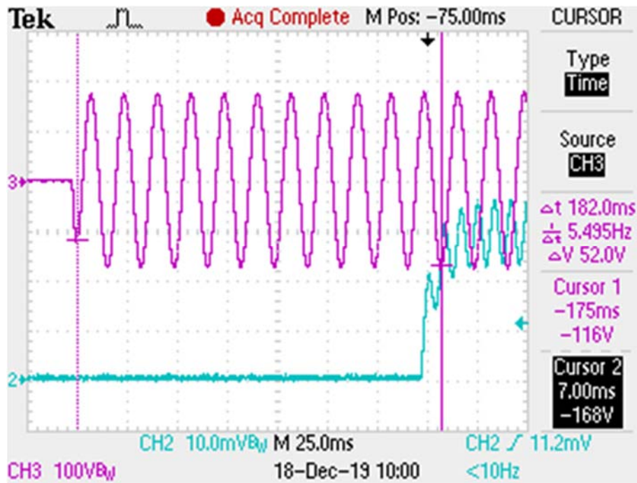
Figure 10. Full Load Start Up with 120 V ac Input
