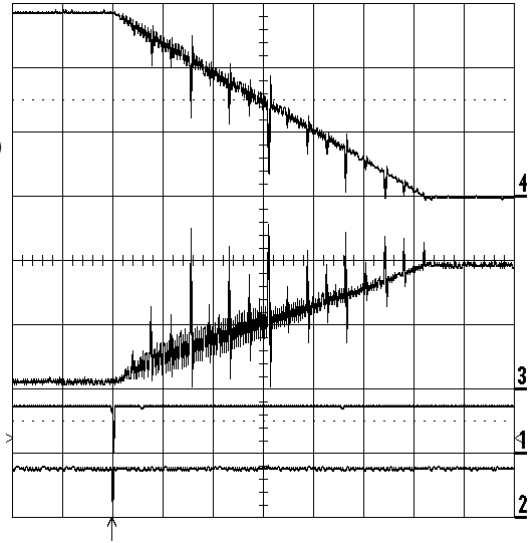
Waveform when it drives from Full code to 0
