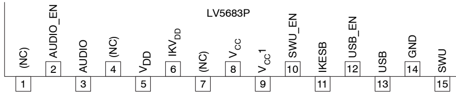
Figure 3. Pin Assignment
