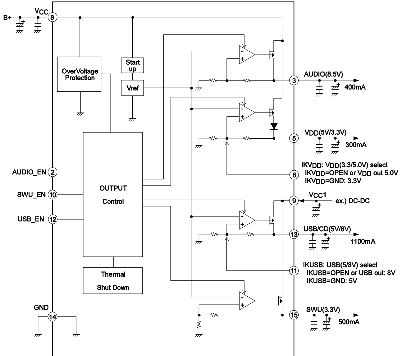
Figure 4. Block Diagram
