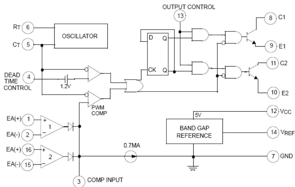
Figure 1. Block Diagram
