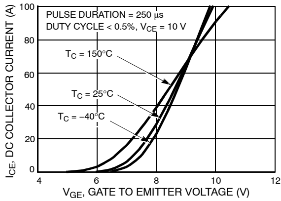
Figure 1. TRANSFER CHARACTERISTICS
