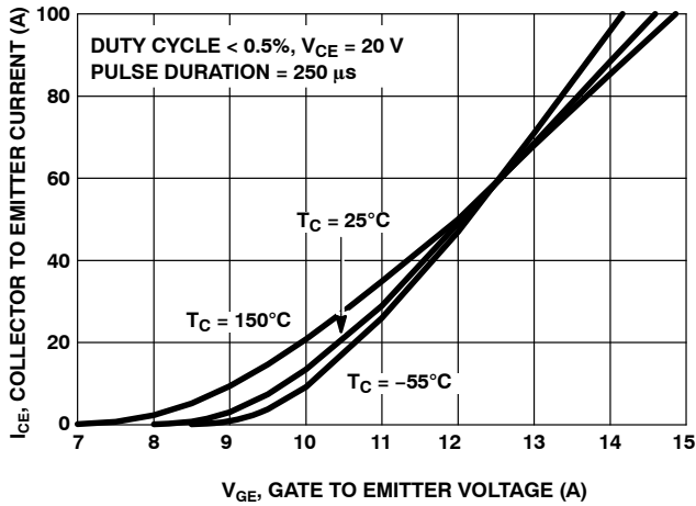
Figure 13. TRANSFER CHARACTERISTIC
