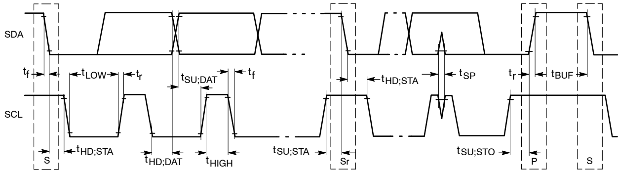
Figure 6. Definition of Timing for Full-Speed Mode Devices on the I²C Bus
