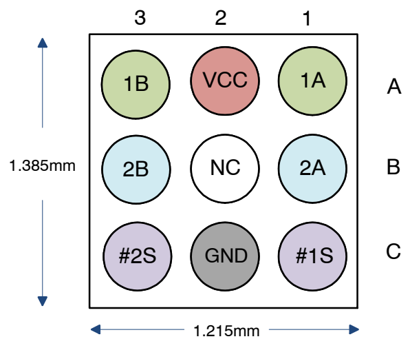
Figure 3. Bottom View
