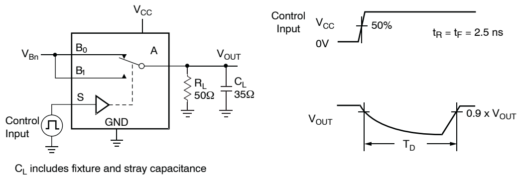
Figure 12. Break-Before-Make Timing
