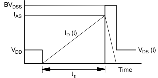
Figure 16. Unclamped Inductive Switching Test Circuit & Waveforms
