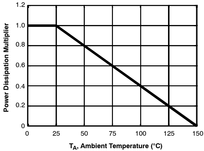
Figure 1. Normalized Power Dissipation vs Ambient Temperature
