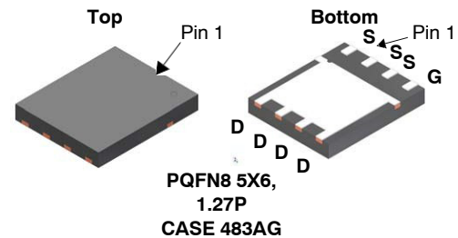
N-CHANNEL MOSFET
