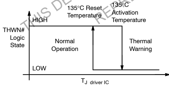
Figure 26. THWN Operation
