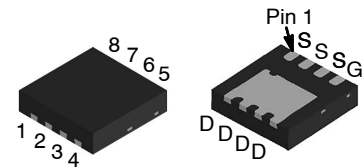
Top Bottom WDFN8 3.3 x 3.3, 0.65P CASE 511DH
