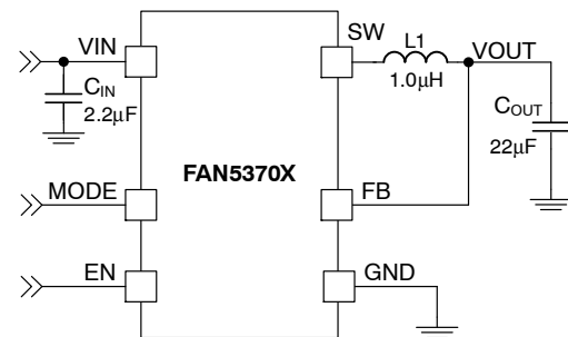
Figure 1. Typical Application
