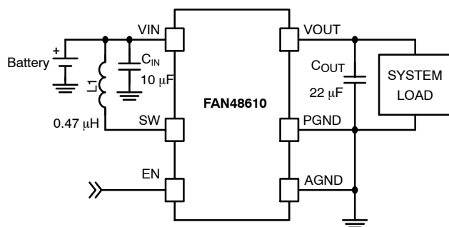
Figure 1. Typical Application
