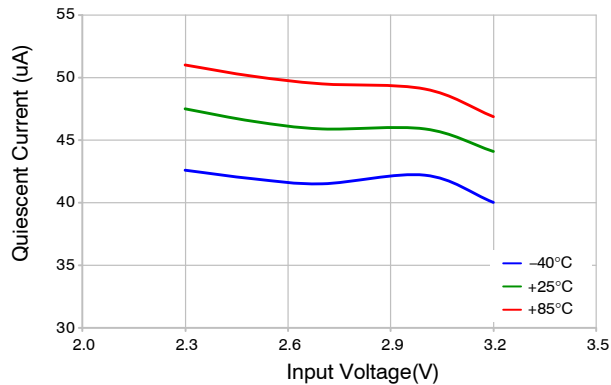
Figure 39. Quiescent Current
