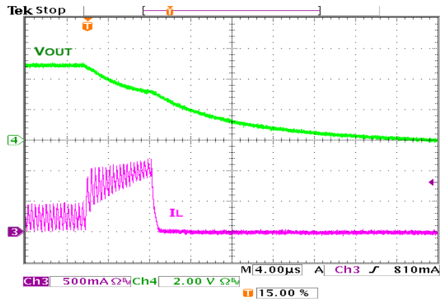
Figure 33. Overload Protection
