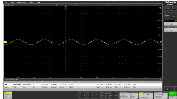
Figure 36. VBUSOUT Ripple for 15 V / 0 A
