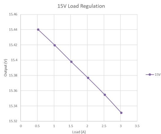
Figure 13. 15 V Regulation
